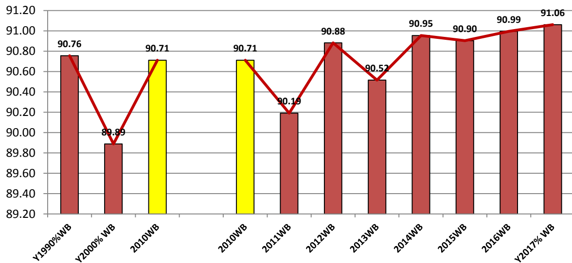
Figure 4. %MEI values of HDI across former USSR countries as from WB data
